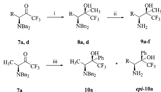
Scheme 6. Reagents and conditions: (i) MeMgBr, Et 2 O, 0 °C. 60% for 8a and 70% for 8d ; (ii) H 2 , Pd(OH) 2 /C, MeOH, room temp., 65% for 9a and 85% for 9d ; (iii) PhMgBr, Et 2 O, 0 °C, 65%, 10a/epi-10a = 72:28
