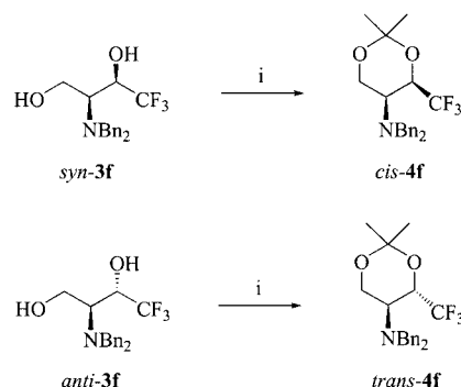
Scheme 2. Reagents and conditions: (i) DMP, TsOH, H 2 O, 60 °C
