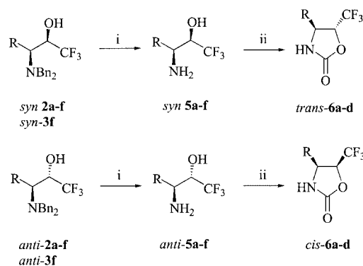
Scheme 3. Reagents and conditions: (i) H 2 , Pd(OH) 2 /C, MeOH; (ii) (CCl 3 O) 2 CO, DIPEA, CH 2 Cl 2 , 0 °C to room temp.
