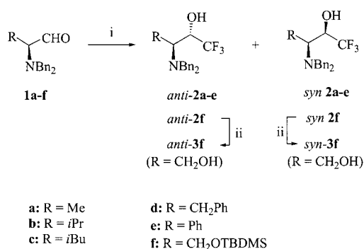
Scheme 1. Reagents and conditions: (i) 1. TMSCF 3 /TBAF, THF, 0 °C; 2. NH 4 Cl/H 2 O; (ii) TBAF (1 equiv.), THF, 0 °C
