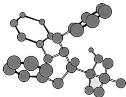
Figure 1. ORTEP representation of X-ray for compound 8d ; for clarity, only H atoms attached to oxygen and C-3 are shown
