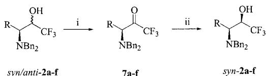
Scheme 4. Reagents and conditions: (i) (COCl) 2 , DMSO, Et 3 N, CH 2 Cl 2 , –78 °C; (ii) NaBH 4 , MeOH/THF, –18 °C
